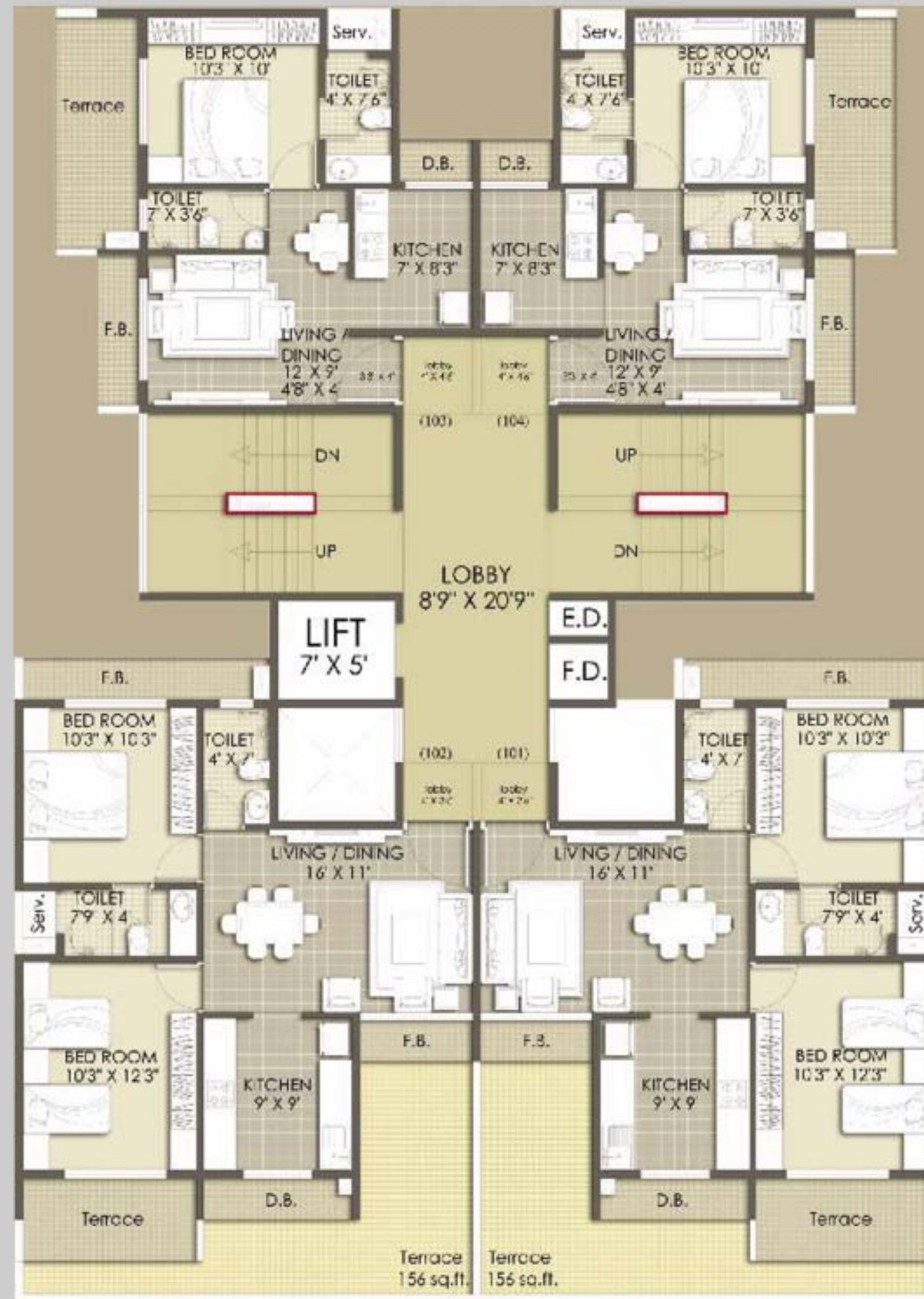
TYPICAL 1 ST FLOOR PLAN
