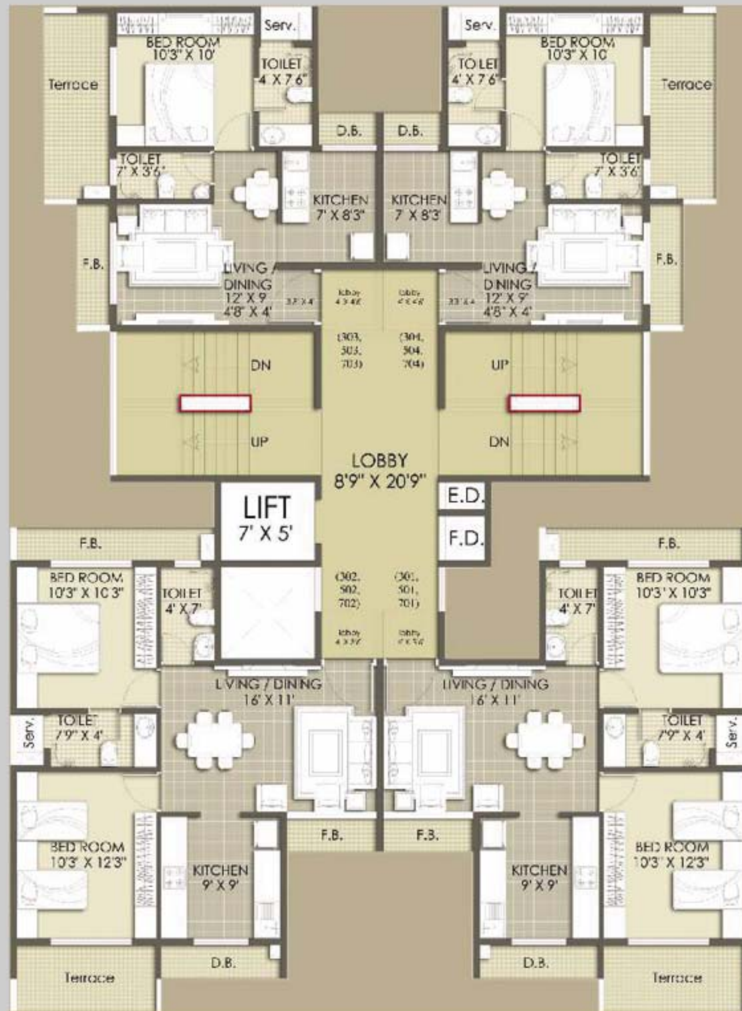
TYPICAL FLOOR PLAN - 3 RD , 5 TH & 7 TH
